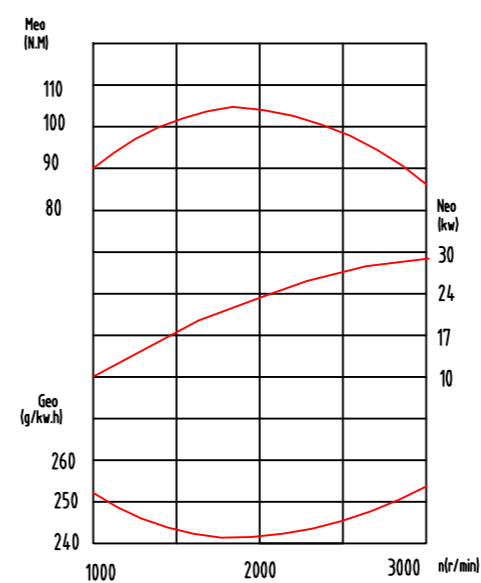
Full speed & full load characteristic curve Model 480 diesel engine
