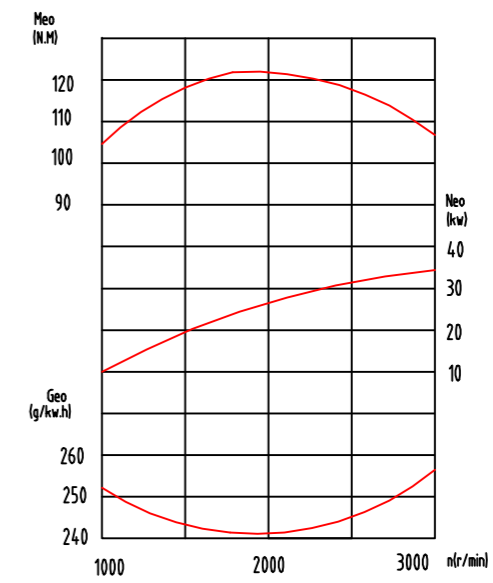
Full speed & full load characteristic curve Model 485 diesel engine
